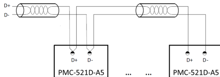
Figure 2-6 RS-485 Connections
