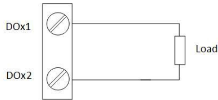
Figure 2-8 DO Connections
