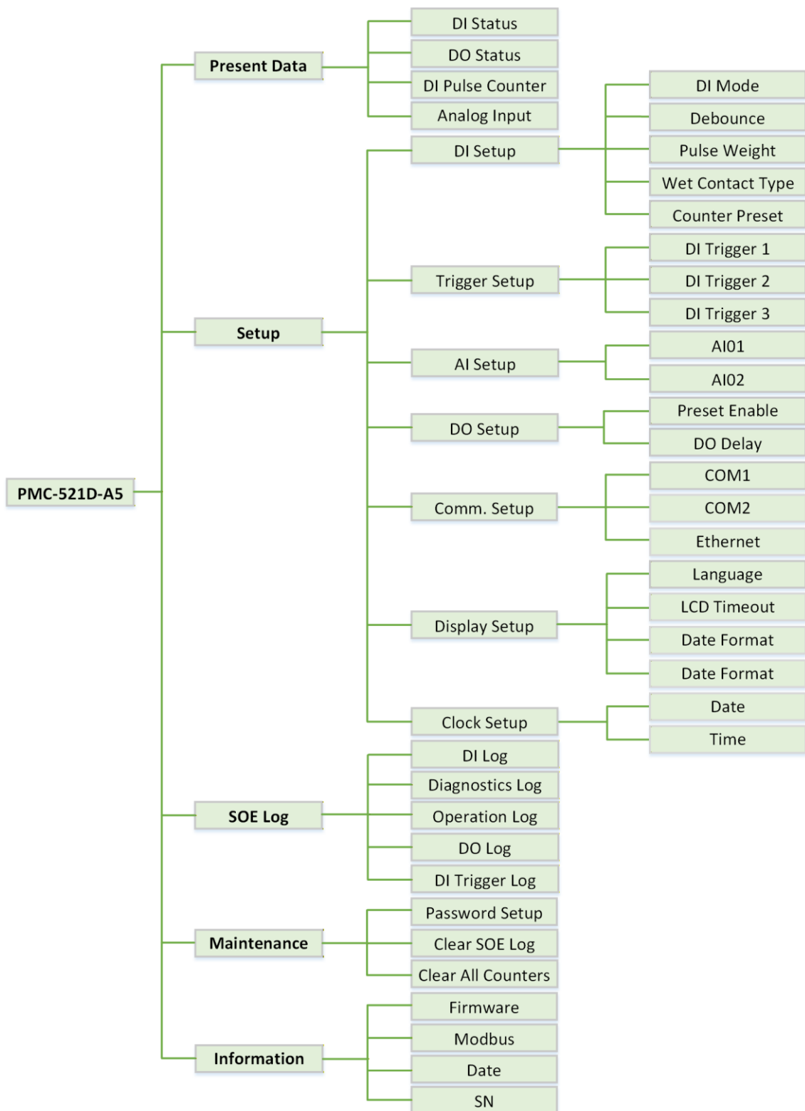
Figure 3-4 PMC-521D-A5 Menu
