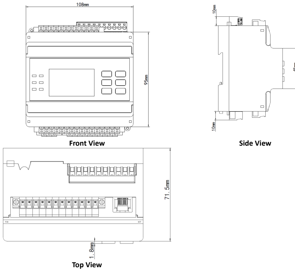
Figure 2-4 Unit Dimensions
